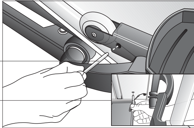
Diagram 24 EFX Locking pin.
